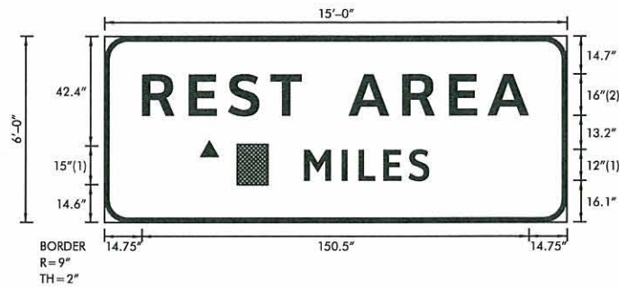
90.00 SQ. FT. BLUE REFLECTORIZED BACKGROUND D5-1
